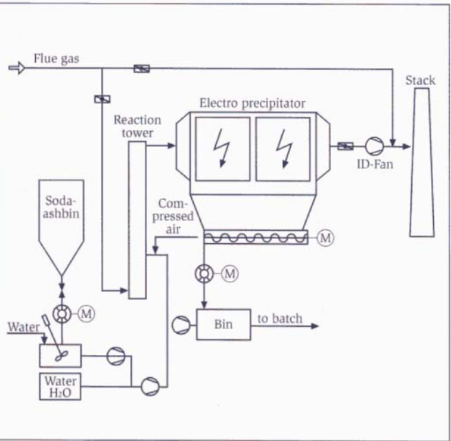
Reactor with Soda/H 2 O-Additiv and Electrostatic Precipitator
