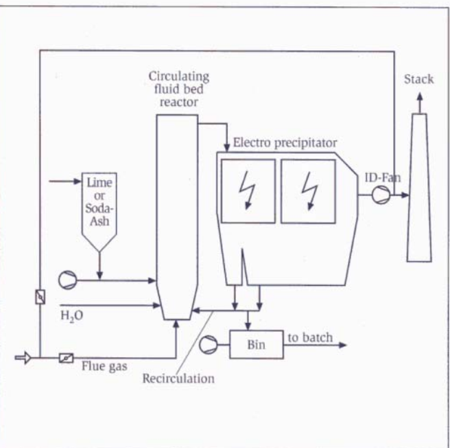
Reactor with circulated Fluid Bed and Electrostatic Precipitator
